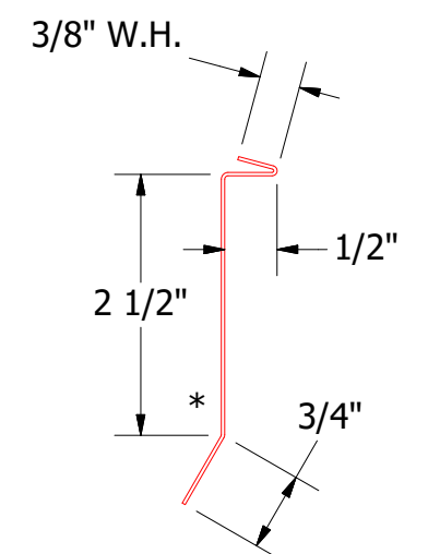
HBA980-Counterflashing
