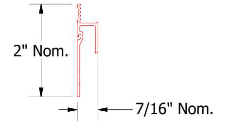
Termination J Molding Extrusion (2) Termination J Molding Extrusion Installed on EJ Sub-Framing Member.
