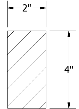
Foam Tape (3b) 4" Foam Tape Strips Installed Vertically on AH Sub-Framing Member. (4) Foam Tape at Center and Adhesive Installed on Both Sides of Tape on SH Sub-Framing Member For Transitions.
