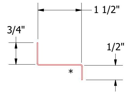
Window Sill Closure Trim
