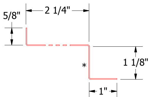
HSA911-Vented Z Closure
