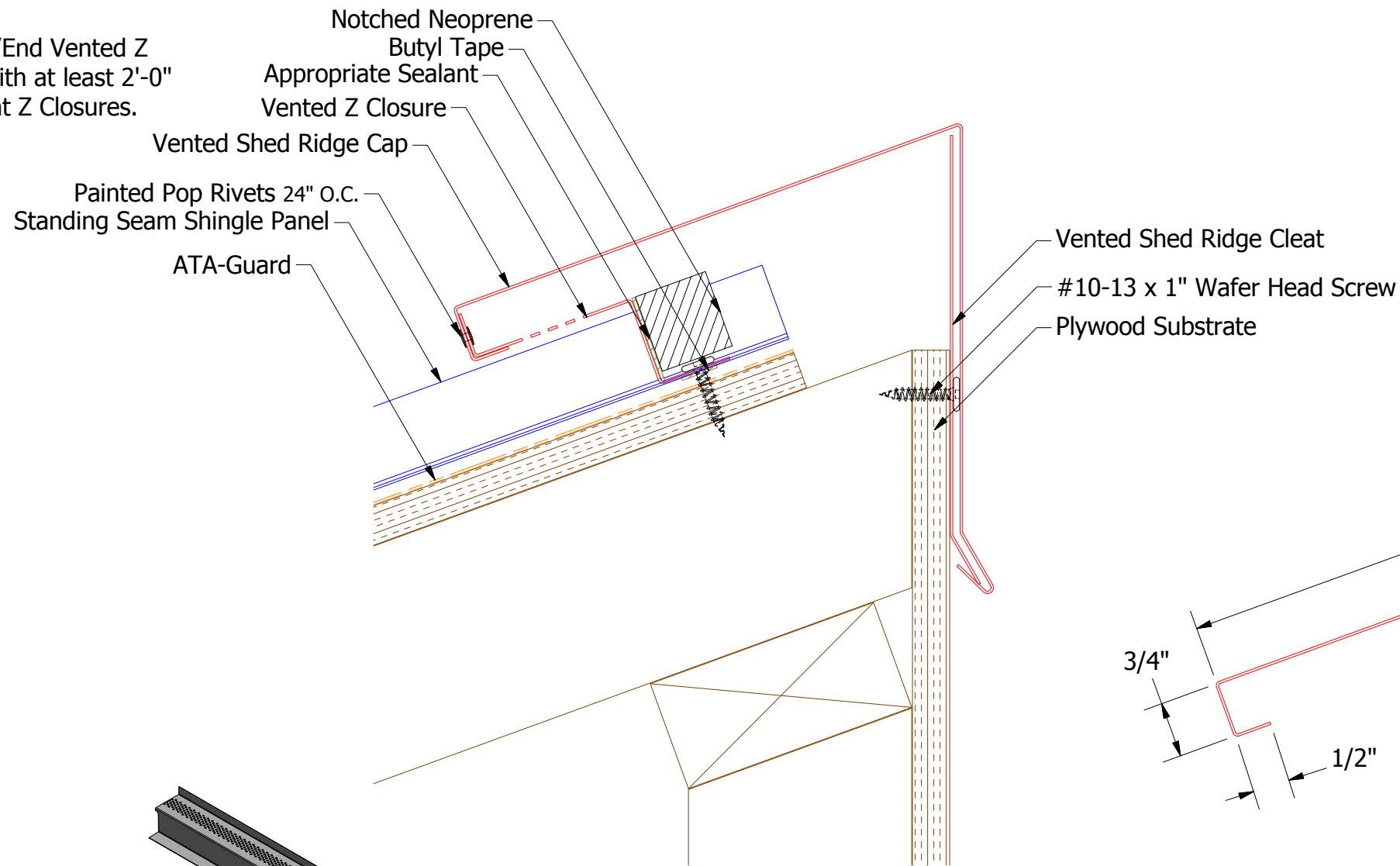
Vented Shed Ridge Cap
