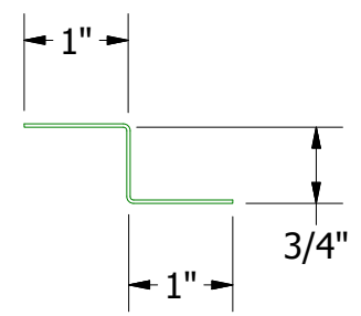
Support Z
