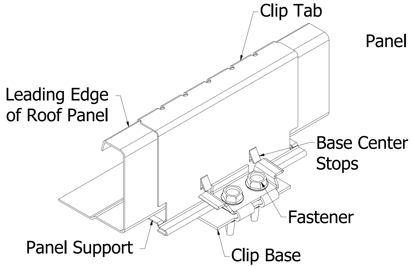
3/8" Stand-Off Clip
