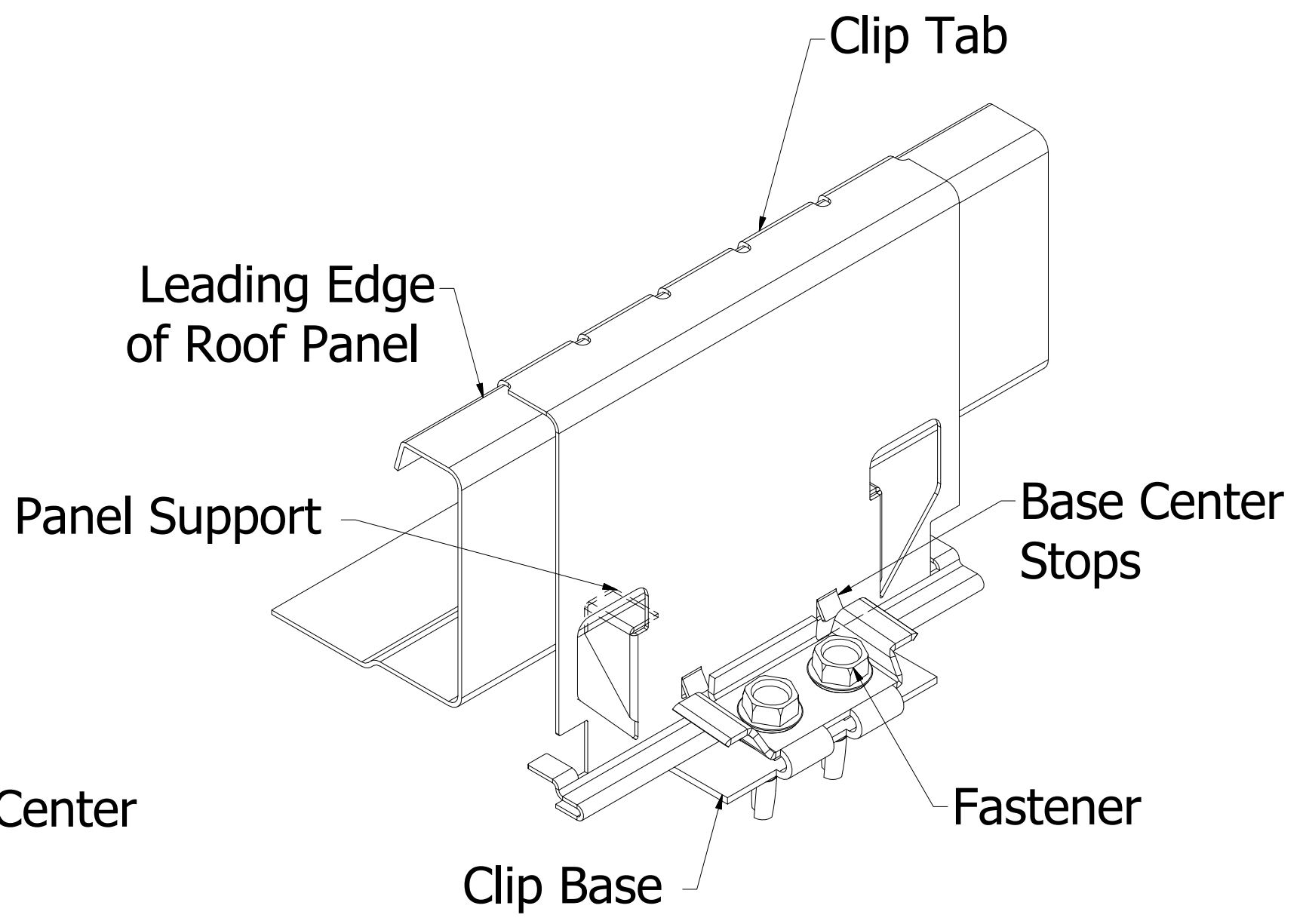
1 3/8" Stand-Off Clip
