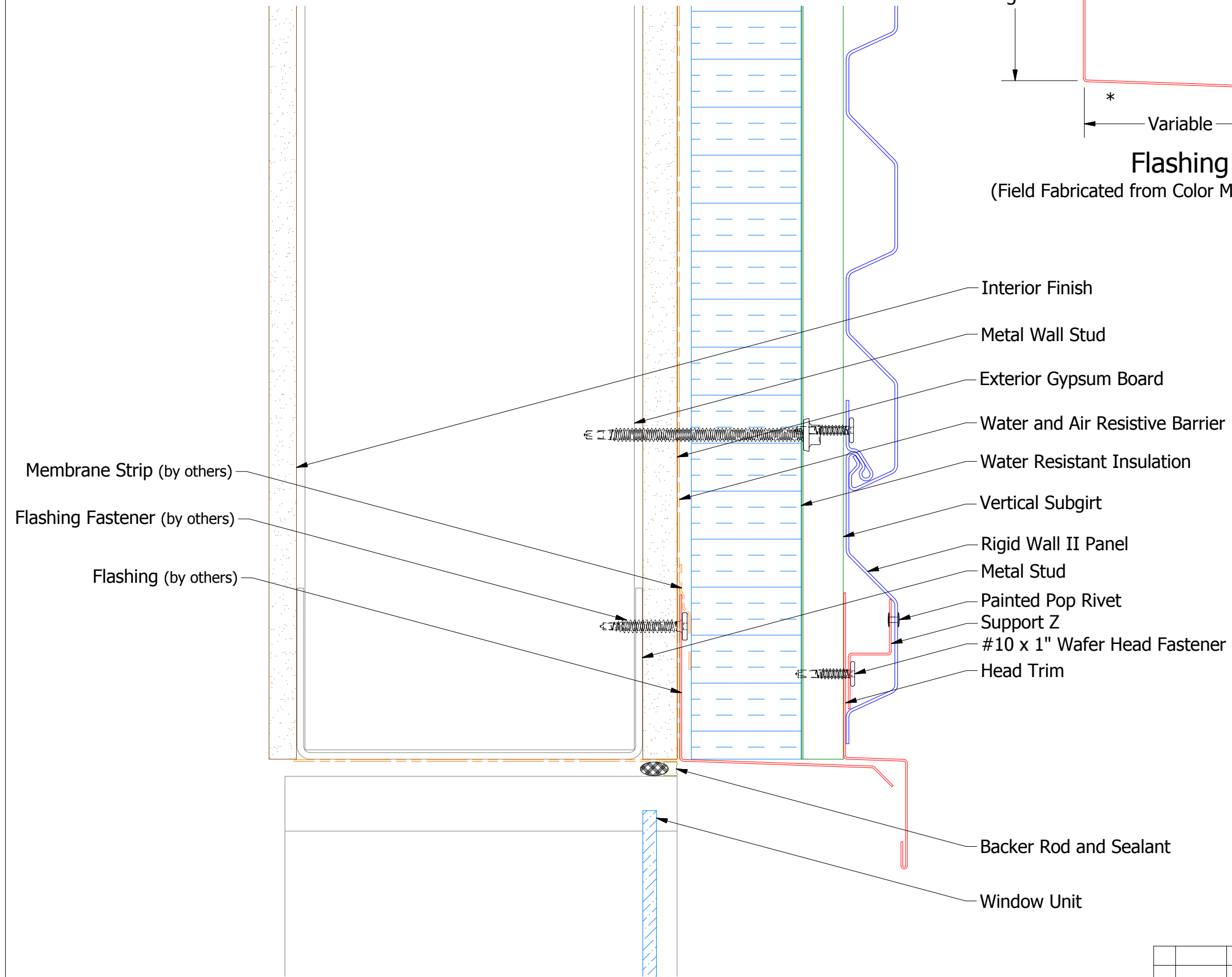
MCA550-Head Trim
