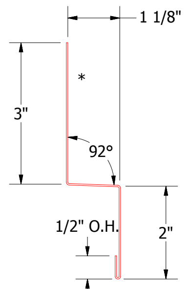
MCA550-Head Trim
