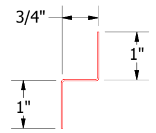
MCA681-Support Z
