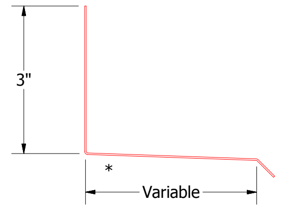
Flashing (Field Fabricated from Color Matched Flat Stock)
