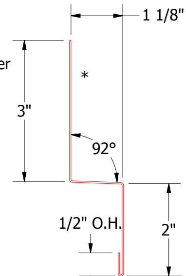
MCA550-Head Trim
