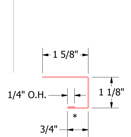
MCA118-J Channel
