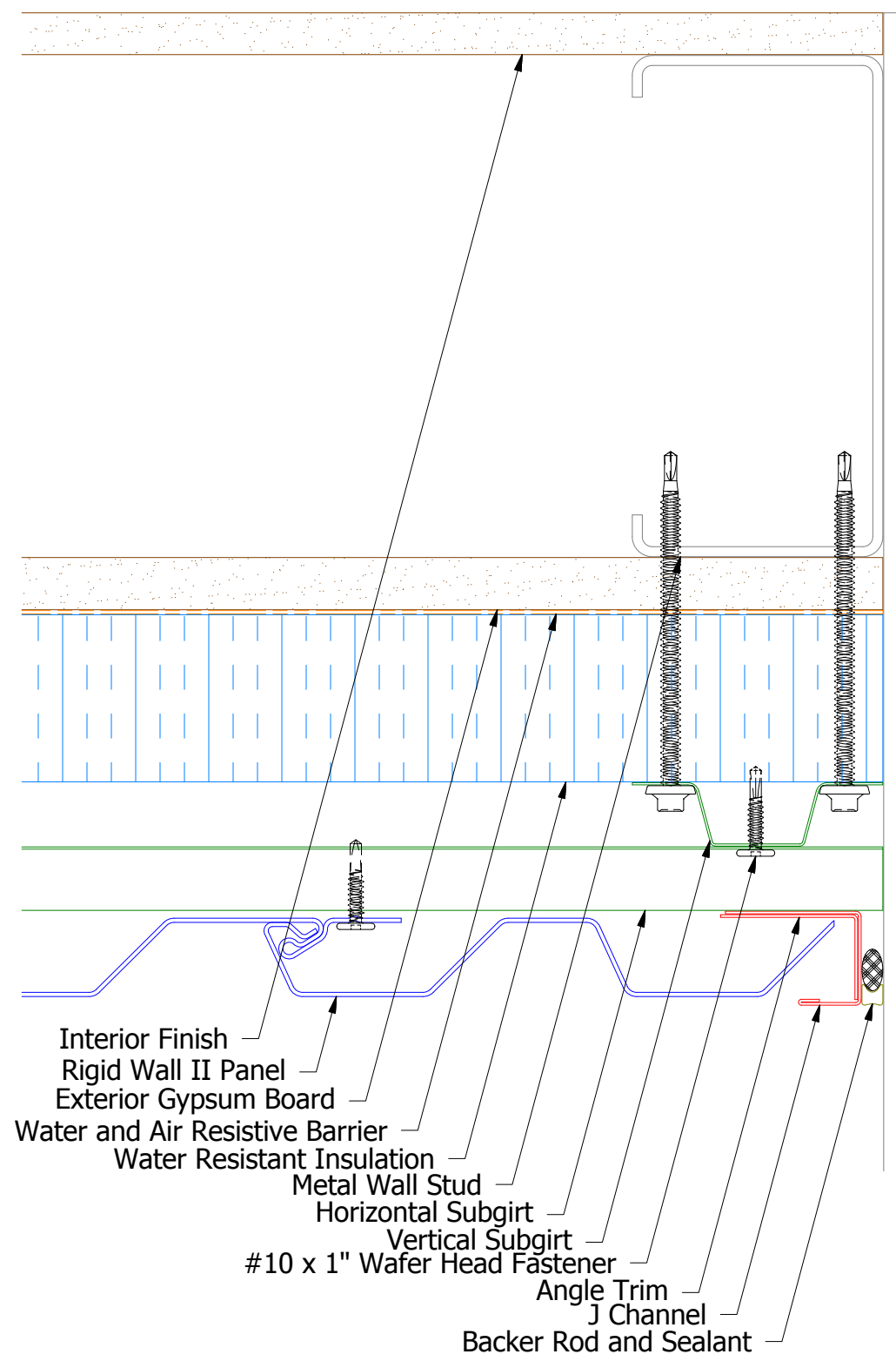
Alternate Subgirt Orientation (NTS)
