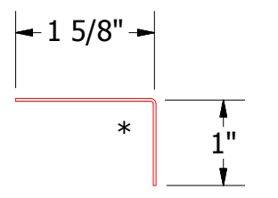
MCA680-Angle Trim
