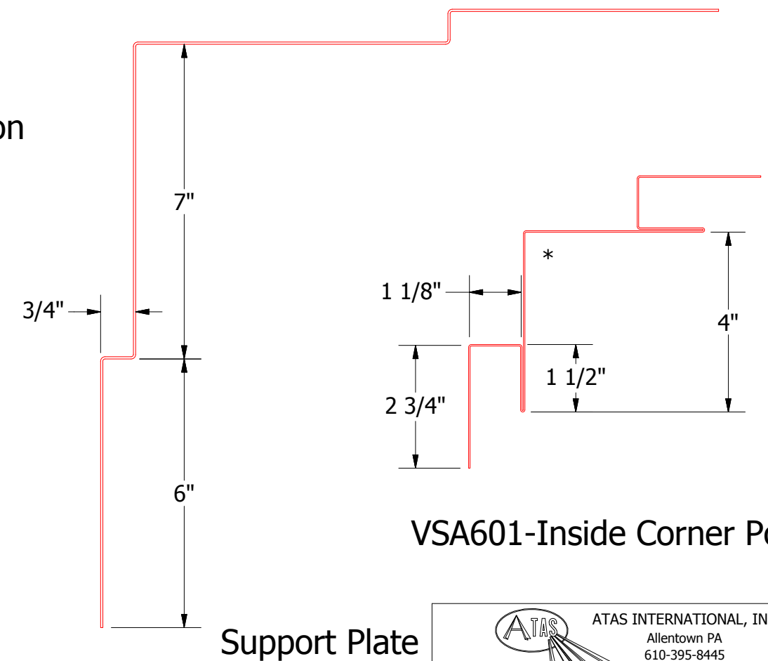
TITLE Versa-Line Open Inside Corner Detail
