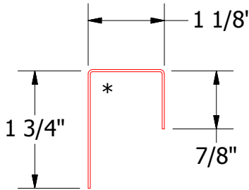
VSA270-J Closure
