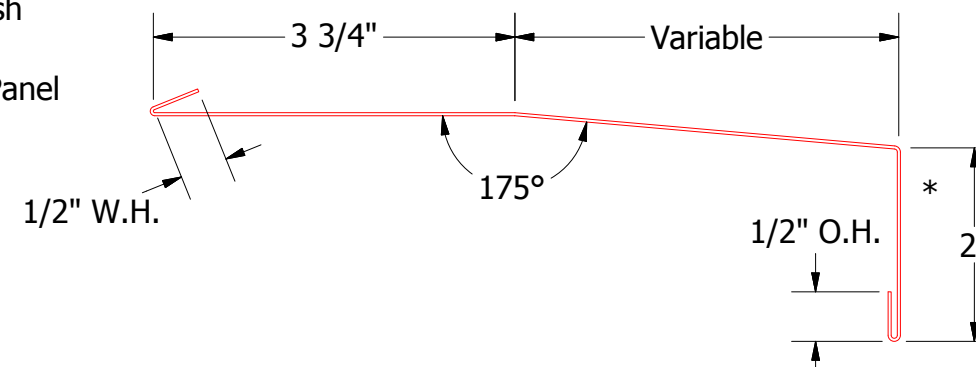
VSA670-Window Sill Trim
