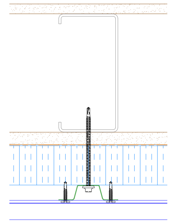
Alternate Subgirt Orientation
