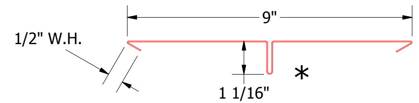
VSA672-Reveal Trim
