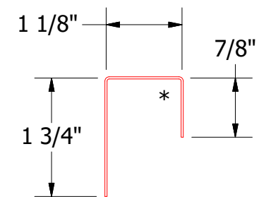
VSA270-J Closure
