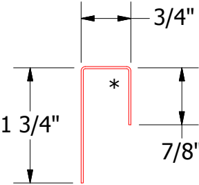
BGA270-J Closure
