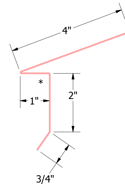
HBA113-Eave Trim
