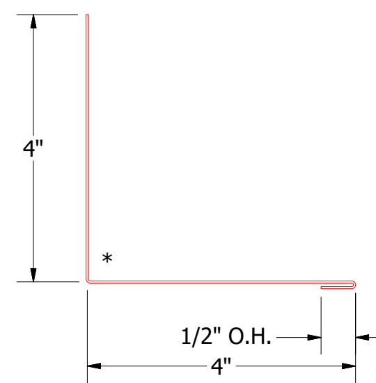
HBA410-Sidewall Trim
