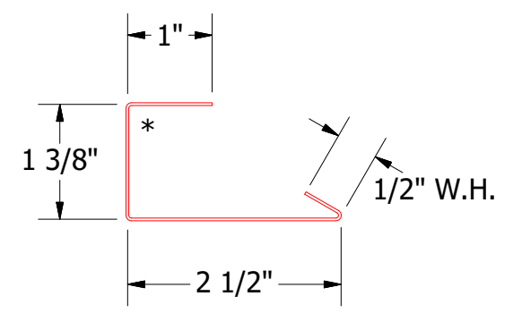
HBA200-Channel Trim
