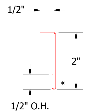
End Flashing
