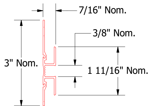
Reveal H Molding Extrusion
