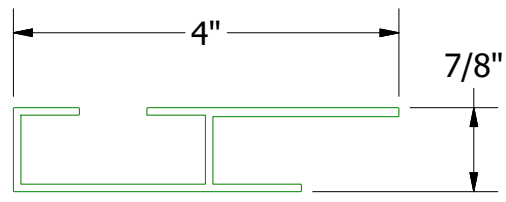
EJ Sub-Framing Member
