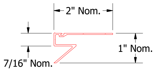
Inside Corner Extrusion
