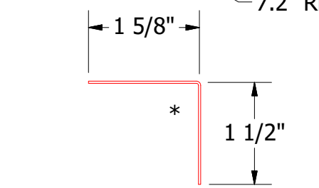
BWA680-Angle Trim
